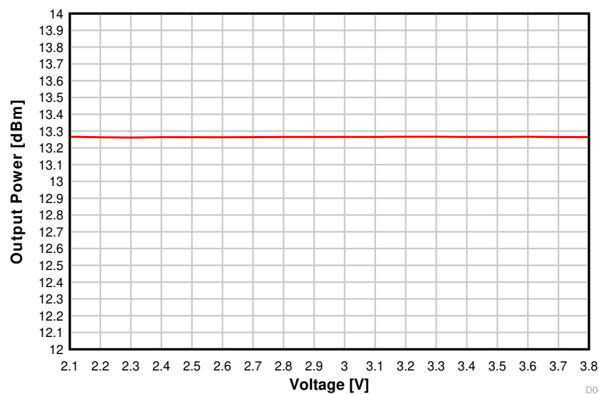
Figure 8-36. Output Power vs. Supply Voltage (VDD5) (50 kbps, 868.3 MHz)
