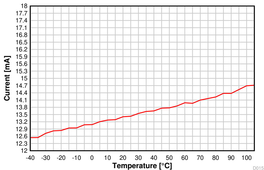
Figure 8-13. TX Current vs. Temperature (50 kbps, 868.3 MHz, VDD = 3.6 V)
