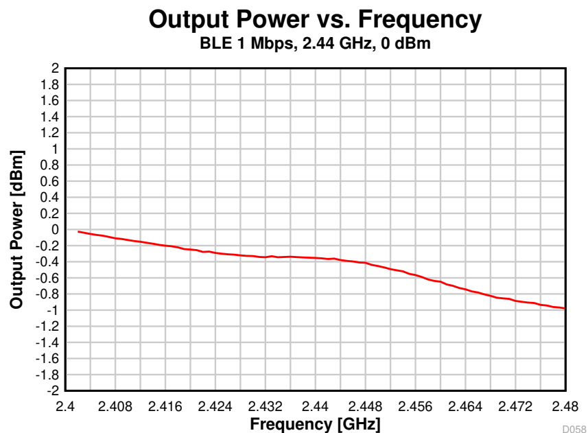
Figure 8-54. Output Power vs. Frequency (BLE 1 Mbps, 2.44 GHz)
