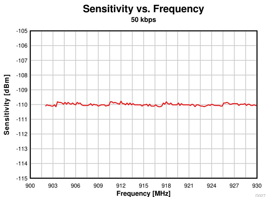
Figure 8-24. Sensitivity vs. Frequency (50 kbps, 915 MHz)
