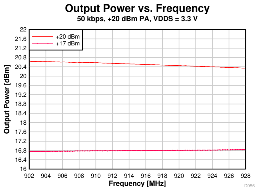
Figure 8-53. Output Power vs. Frequency (50 kbps, 915 MHz, VDDS = 3.3 V)
