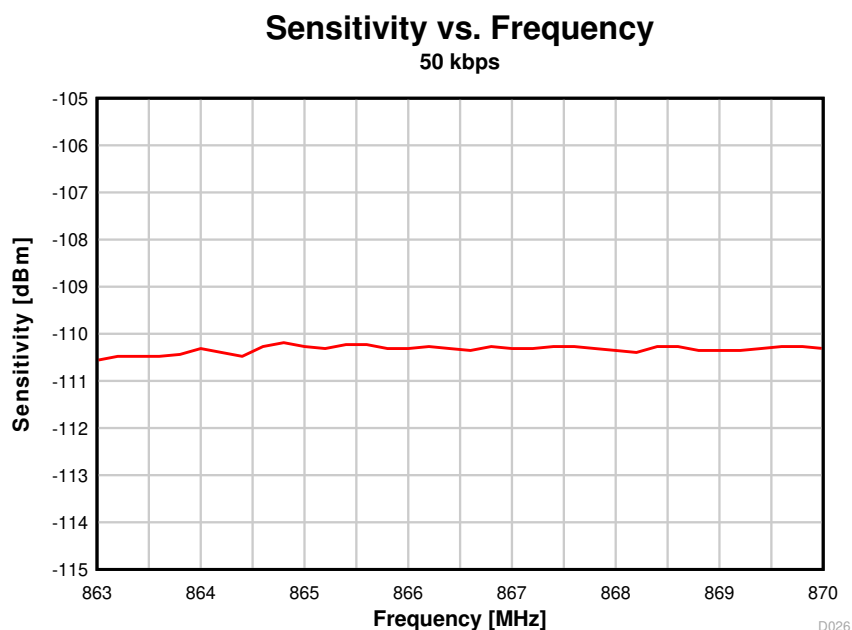
Figure 8-23. Sensitivity vs. Frequency (50 kbps, 868 MHz)
