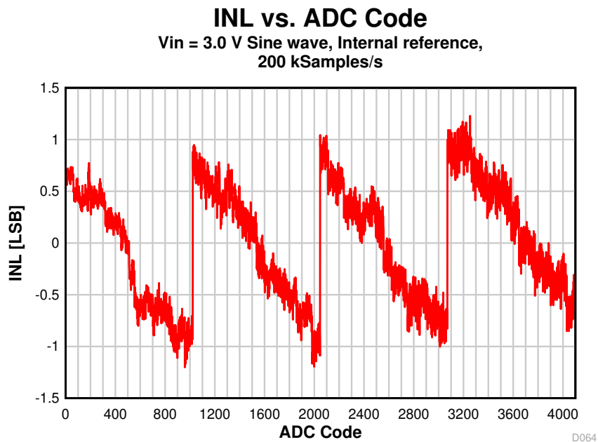
Figure 8-60. INL vs. ADC Code
