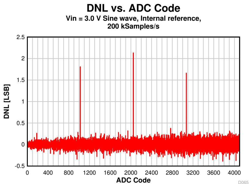
Figure 8-28. DNL vs. ADC Code
