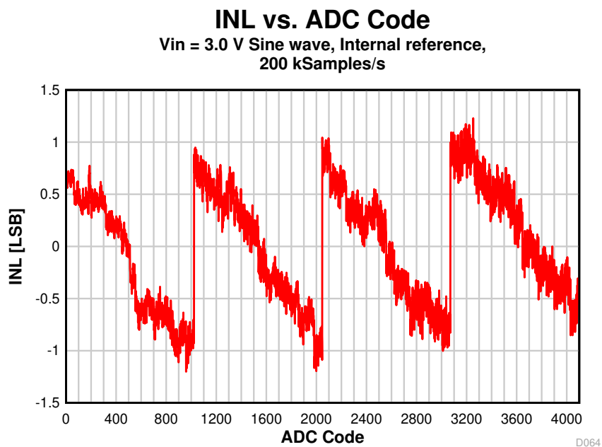
Figure 8-27. INL vs. ADC Code
