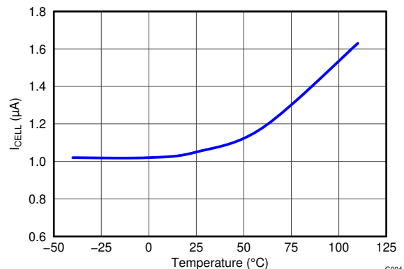
Figure 9-6. I_{CELL} vs. Temperature at V_{CELL} = 9.2 V
