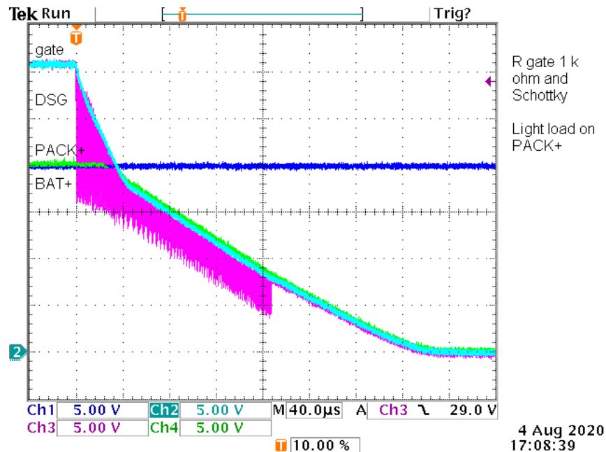
Figure 8-8. Moderate Speed DSG FET Turn-Off, Using a 1-k \Omega Series Gate Resistor, and a Light Load nPACK+.
