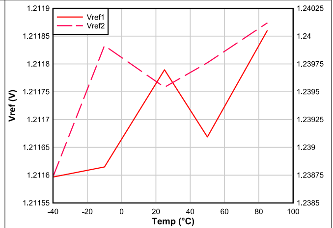
Figure 6-10. Internal Voltage References vs Temperature (VREF1 and VREF2)
