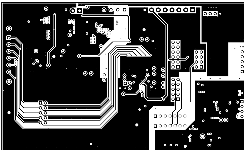
Figure 10-5. BQ76922EVM Layer 3
