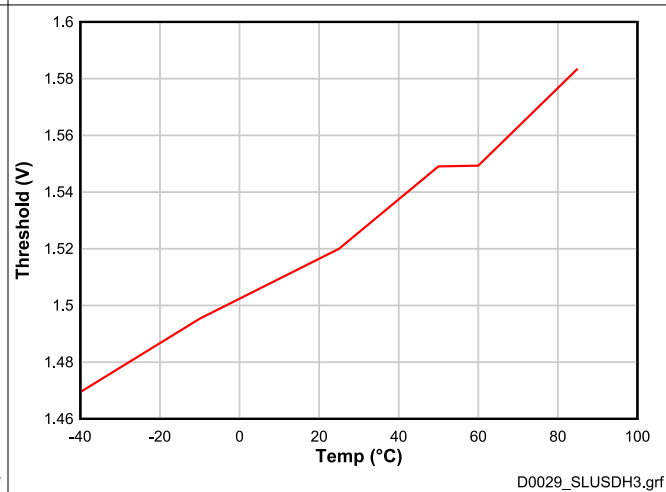
Figure 6-22. LD Wake Voltage vs Temperature
