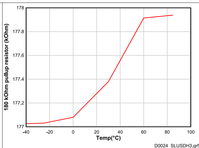
Figure 6-20. Thermistor Pullup Resistance vs Temperature (180-kΩ Setting)
