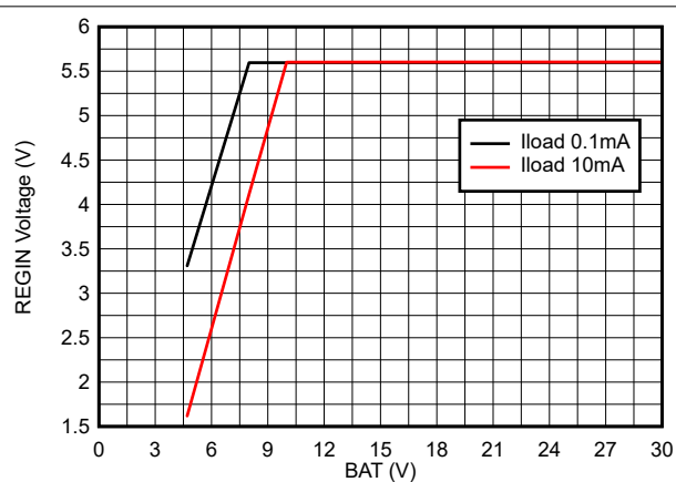
Figure 6-24. RGIN Voltage vs BAT Voltage
