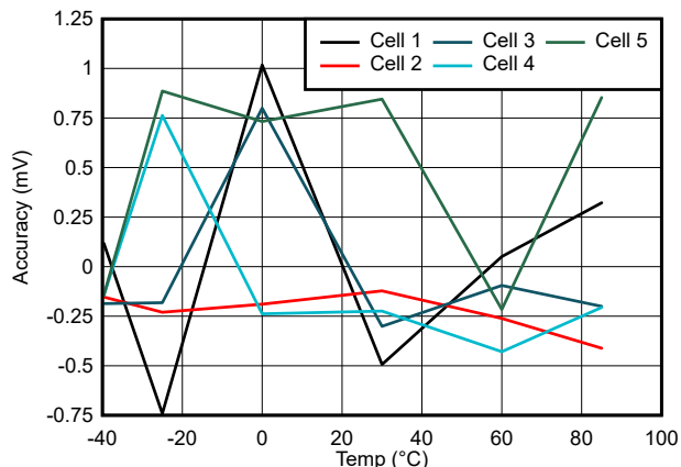
Figure 6-4. Cell Voltage Measurement Error vs Temperature with Cell Voltage = 1.5 V
