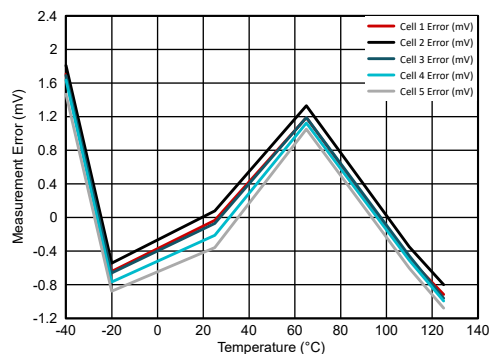
Figure 6-13. Cell Voltage Measurement Error vs. Temperature with Cell Voltage = 5.5 V
