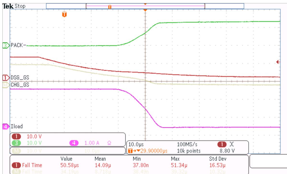
Figure 8-7. A Slower Turn-Off Case Using a 4.5-k \Omega Series Gate Resistor
