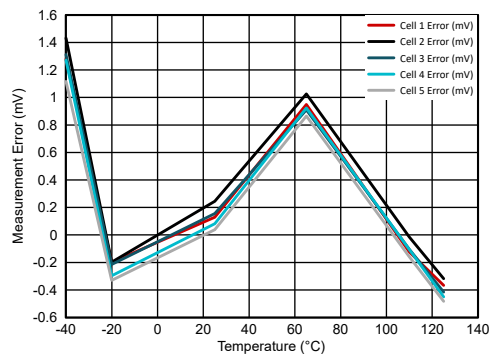
Figure 6-9. Cell Voltage Measurement Error vs. Temperature with Cell Voltage = 3.5 V
