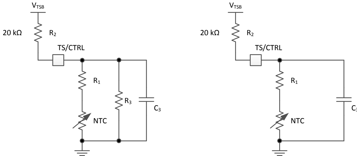
Figure 9-12. NTC Circuit Options For Safe Operation of the Wireless Receiver Power Supply
