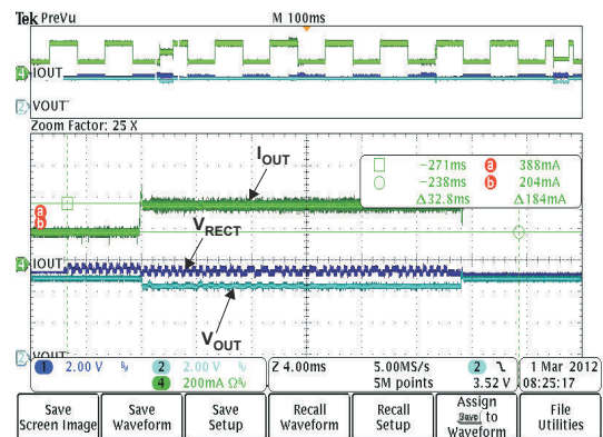
Figure 8-18. Adaptive Communication Limit Event Where the 400-mA Current Limit is Enabled ( I_{OUT-DC} < 300\text{ mA} )
