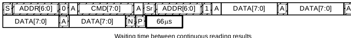
Figure 9. I 2 C Command Waiting Time
