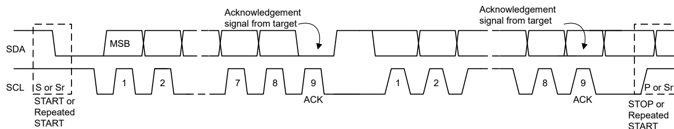
Figure 8-10. Data Transfer on the I²C Bus
