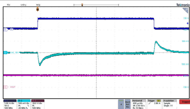
Figure 9-16. Reverse Mode Buck-Boost Transient Response
