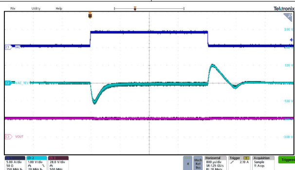
Figure 9-15. Reverse Mode Buck Transient Response
