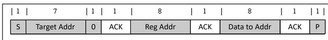
Figure 8-12. Single Write
