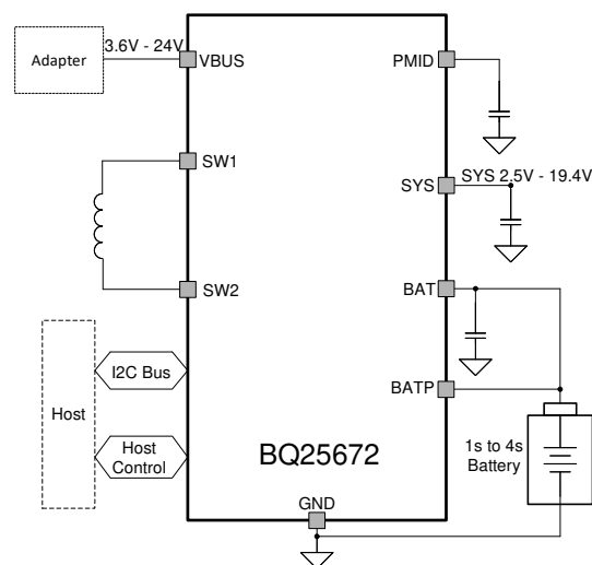
Simplified Schematic
