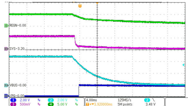
Figure 9-3. Power-Down
