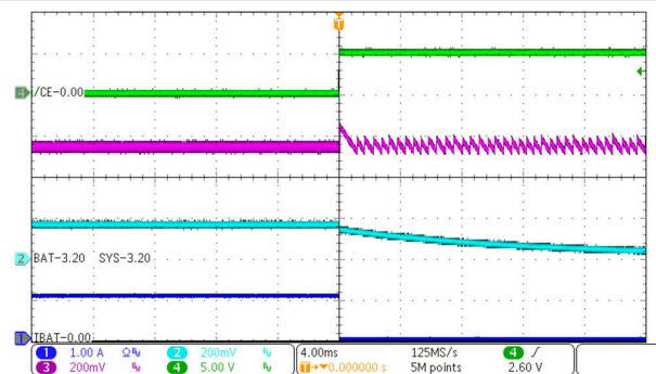
Figure 9-3. Power-Down
