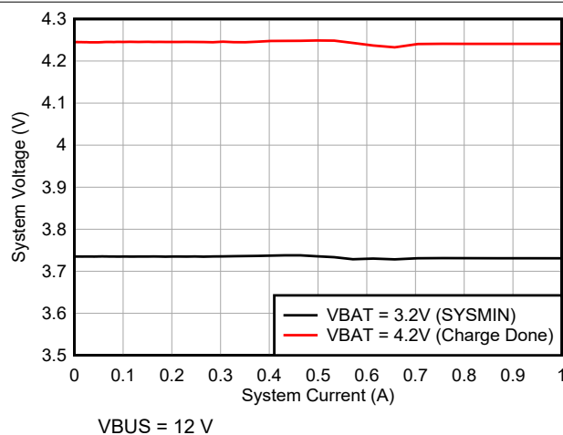
Figure 7-5. System Load Regulation for SYSMIN and After Charge Done
