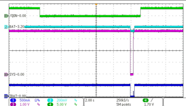
Figure 9-5. Charge Disable
