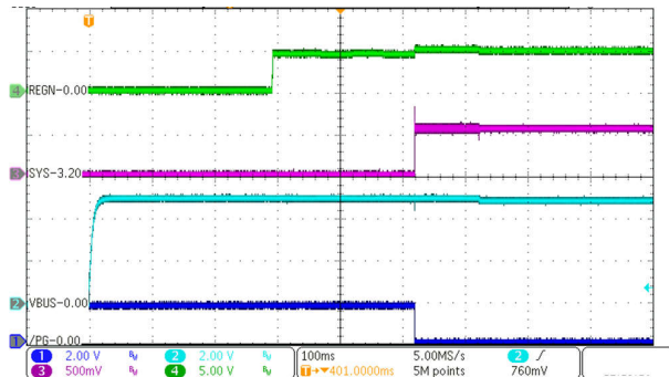
Figure 9-2. Power-Up with Charge Enabled
