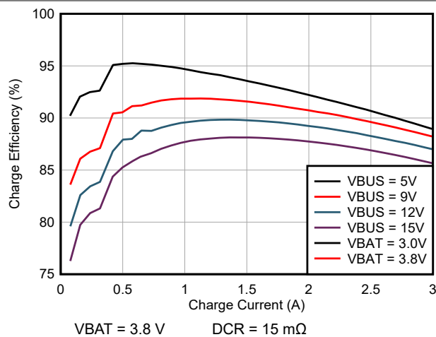
Figure 7-1. Charge Efficiency vs Charge Current
