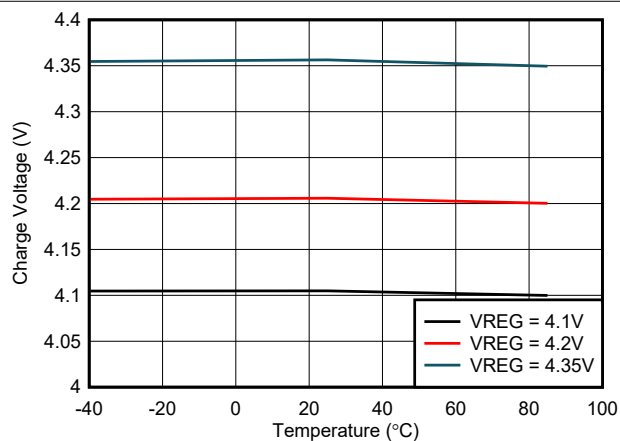
Figure 7-4. Charge Voltage Accuracy vs VREG Setting
