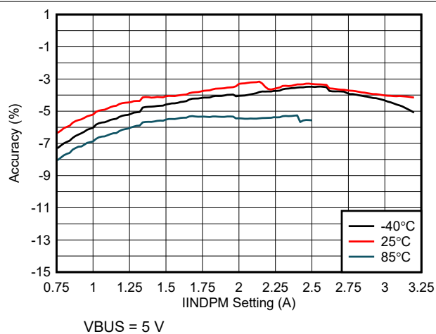
Figure 7-6. Input Current Regulation Accuracy vs IINDPM Setting
