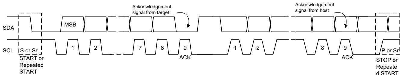
Figure 8-9. Data Transfer on the I²C Bus
