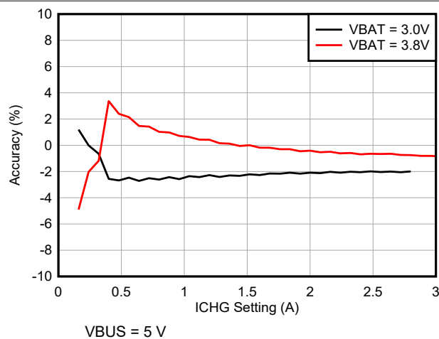
Figure 7-3. Charge Current Accuracy vs ICHG Setting
