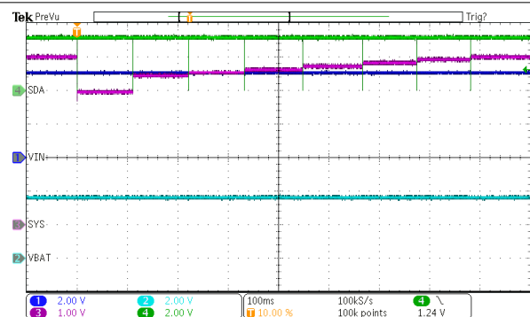
Figure 8-13. SYS Regulation Sweep
