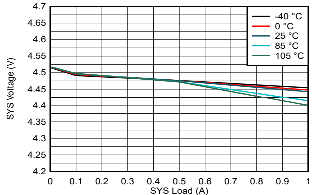
Figure 6-4. SYS Load Regulation
