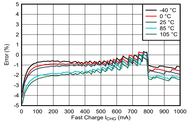
Figure 6-2. Charge Current Accuracy vs ICHARGE Setting
