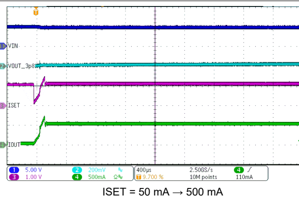
Figure 8-11. ISET Change Response
