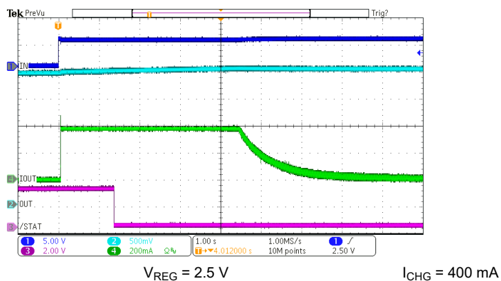
Figure 8-12. Charge Complete
