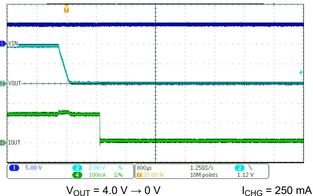
Figure 8-9. OUT Short-Circuit Response
