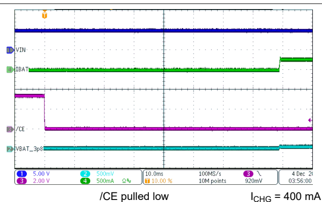
Figure 8-5. Charge Enable
