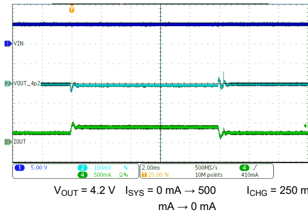
Figure 8-8. OUT Transient Response
