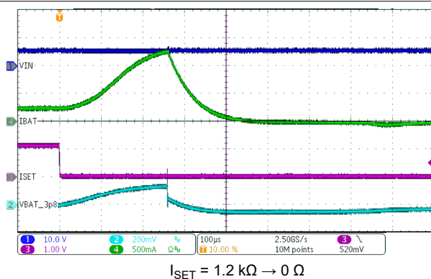
Figure 8-10. ISET Short-Circuit Response
