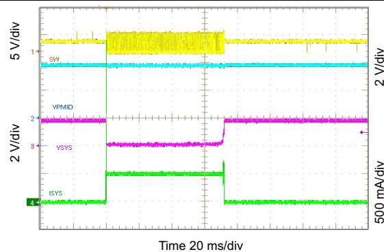
Figure 76. 3.3 V_{SYS} Load Transient, 0 to 200 mA
