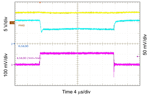
Figure 89. 2.5 V LSLDO Load Transient, 0 to 100 mA
