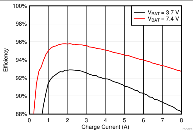
Figure 5-3. Efficiency During Charging
