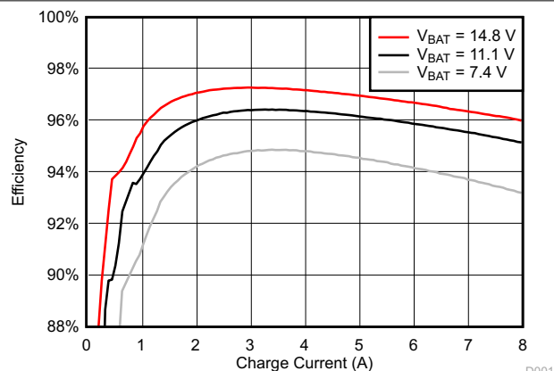
Figure 5-2. Efficiency During Charging
