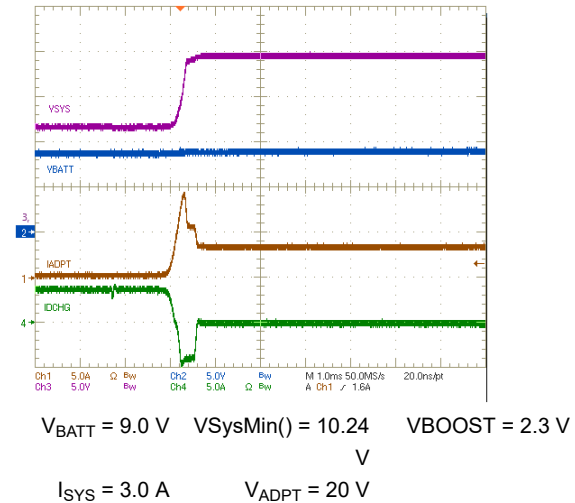
Figure 7-21. Battery Only Boost Exit by Adapter Plug In
