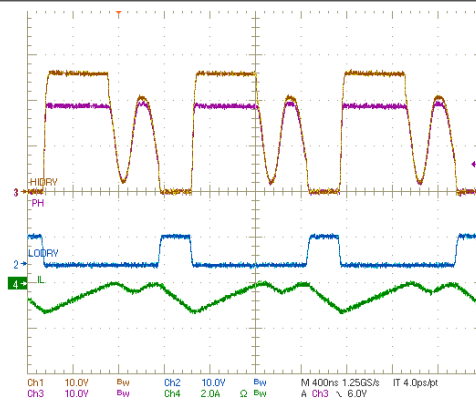
Figure 7-11. Converter in Discontinuous Conduction Mode (DCM) During Charging
