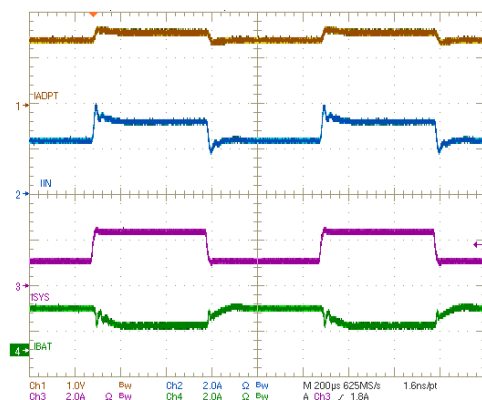
Figure 7-14. Input Current Regulation During System Load Transient
