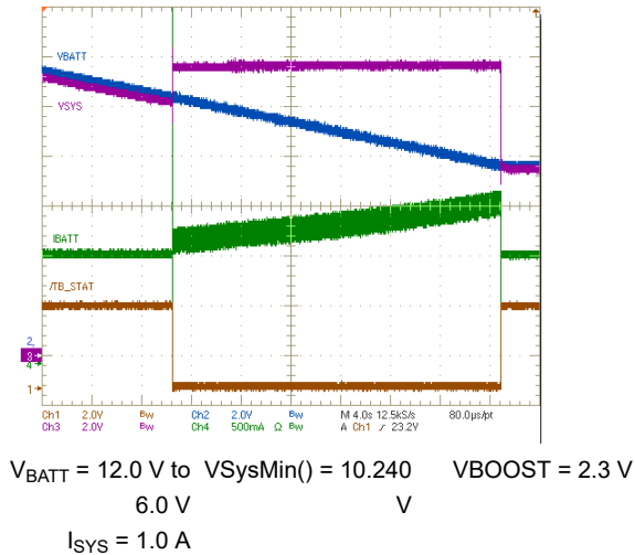
Figure 7-20. Battery Only Boost Entry and Exit by Battery Voltage
