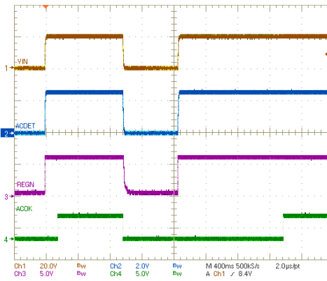
Figure 7-5. Power On ACOK Delay at 1 st and 2 nd Adapter Plug-in
