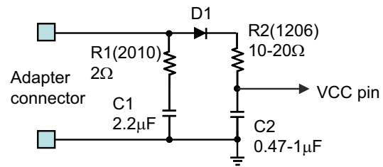
Figure 7-3. Input Filter
