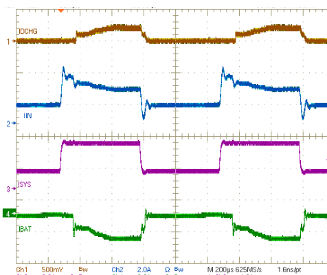
Figure 7-13. Converter in Discontinuous Conduction Mode During Hybrid Power Boost Mode
