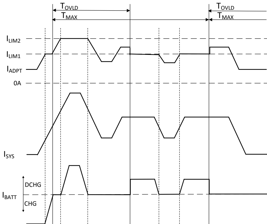
Figure 6-2. Two-Level Adapter Current Limit Timing Diagram, REG0x37[8] = 0
