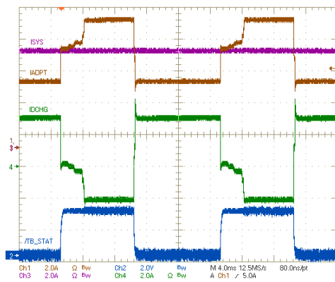
Figure 7-17. Hybrid Power Boost Mode With Discharge Current Regulation
