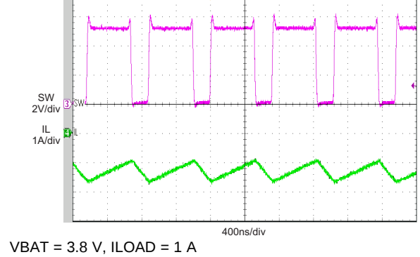
Figure 47. Boost Mode Switching
