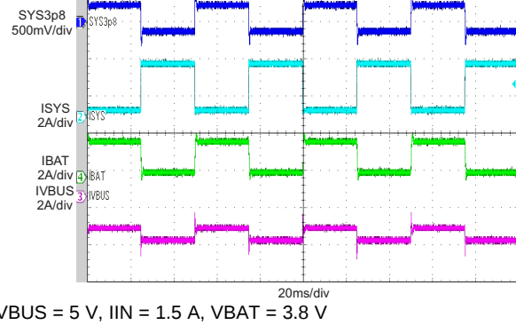
Figure 46. Load Transient During Supplement Mode
