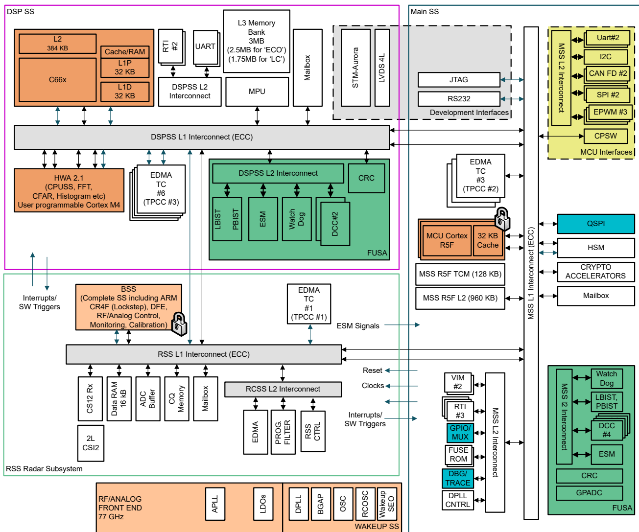
Figure 8-5. Processor Subsystem
