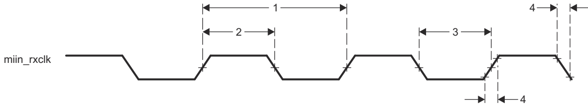
Figure 7-19. Clock Timing (MAC Receive) - MIn operation
