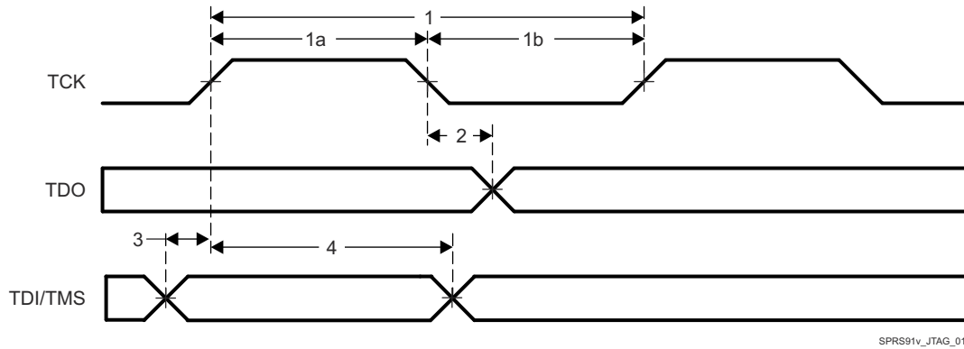
Figure 7-25. JTAG Timing
