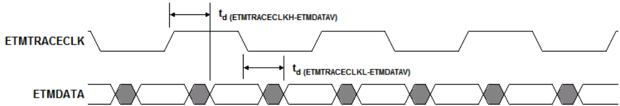
Figure 7-27. ETMDATA Timing
