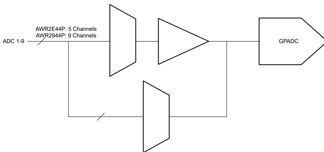
Figure 8-6. GPADC Path
