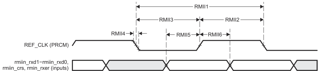
Figure 7-15. MAC Receive Interface Timing, RMII operation
