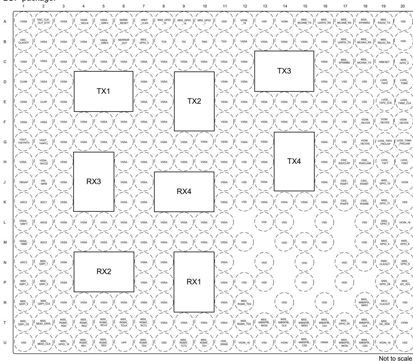
Figure 6-2. Pin Diagram - AWR2E44P/AWR2E44-ECO/AWR2E44LC
