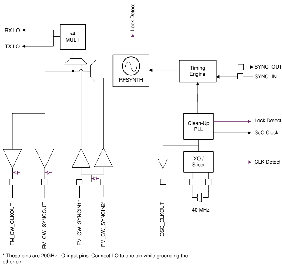
Figure 8-1. Clock Subsystem
