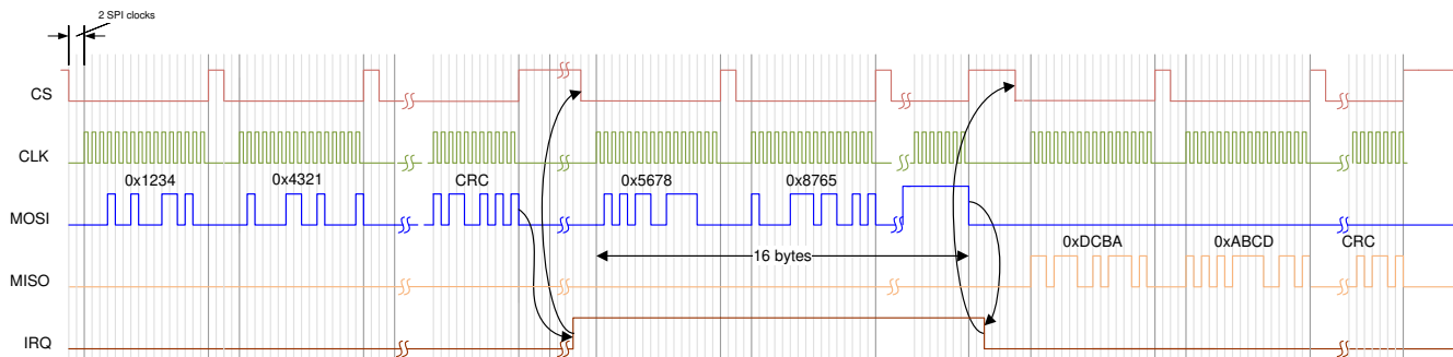
Figure 7-10. SPI Communication
