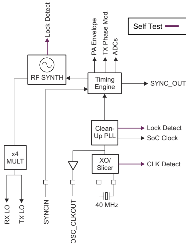
Figure 8-2. Clock Subsystem
