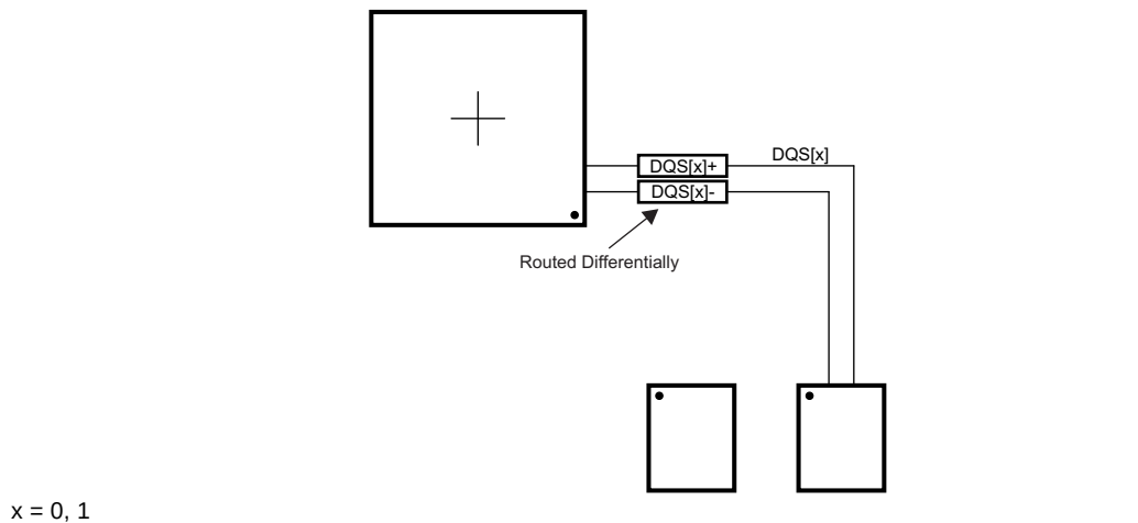
Figure 7-64. DQS[x] Routing With Any Number of Allowed DDR3 Devices
