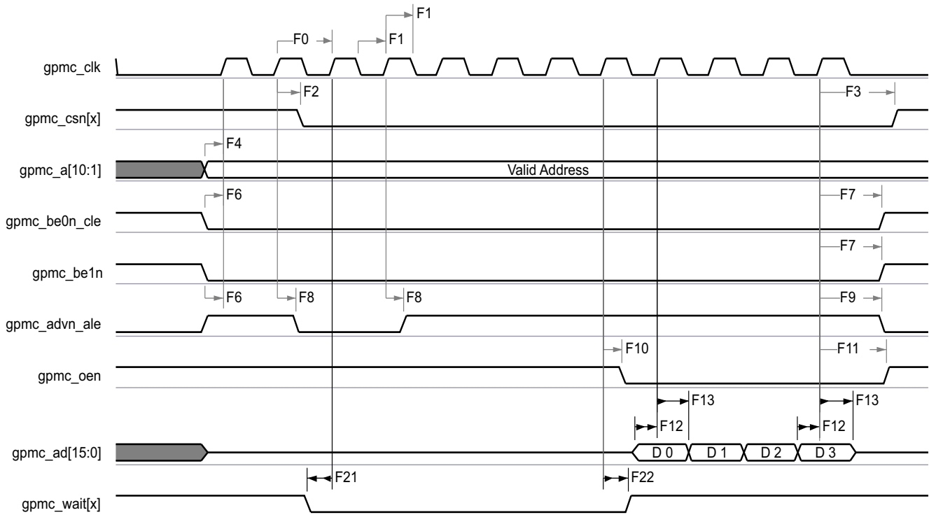
Figure 7-18. GPMC and NOR Flash—Synchronous Burst Read—4x16-Bit (GpmcCLKDivider = 0)
