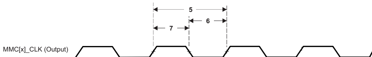
Figure 7-78. MMC[x]_CLK (Output)
