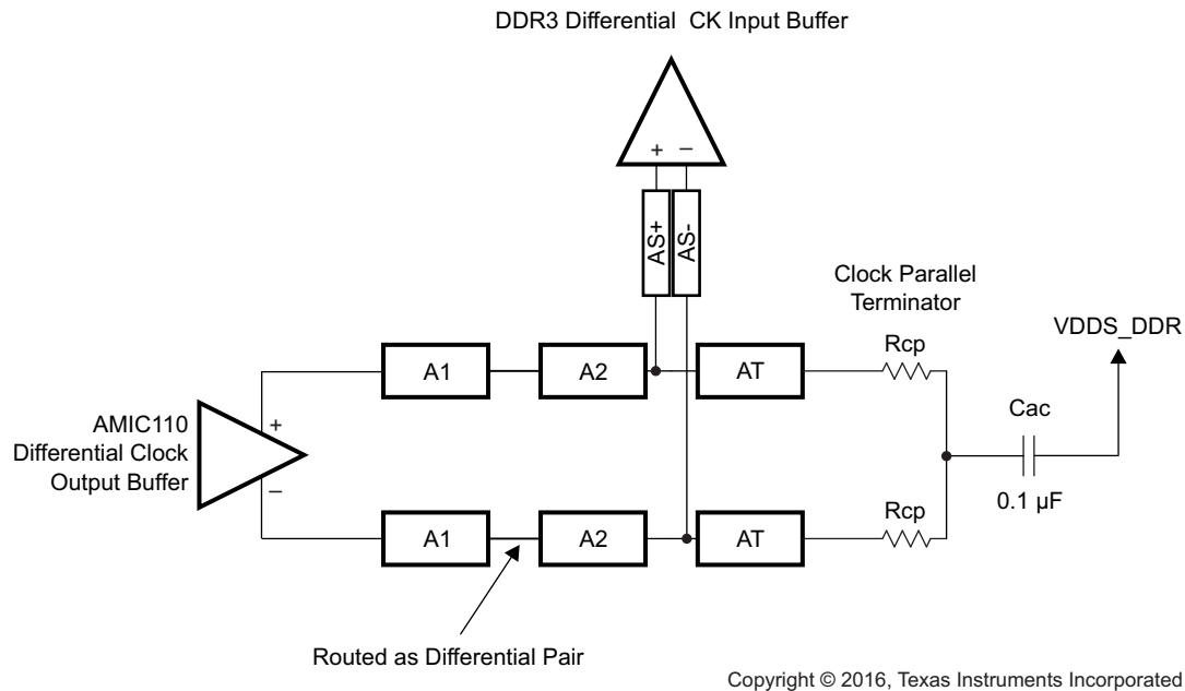
Figure 7-58. CK Topology for One DDR3 Device
