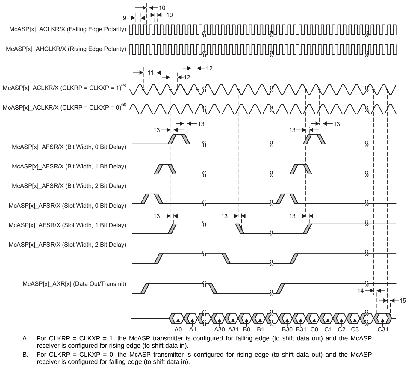
Figure 7-72. McASP Output Timing
