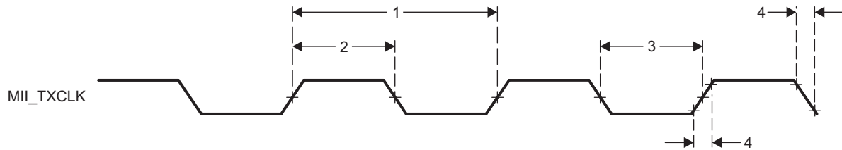
Figure 7-95. PRU-ICSS MII_TXCLK Timing
