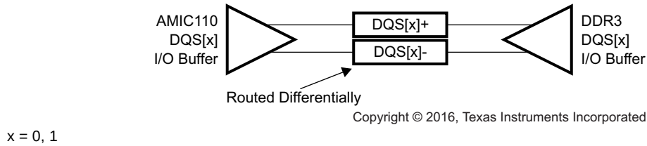
Figure 7-62. DQS[x] Topology
