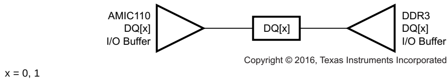
Figure 7-63. DQ[x] Topology
