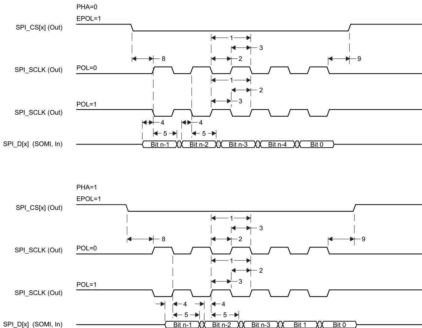
Figure 7-75. SPI Master Mode Receive Timing
