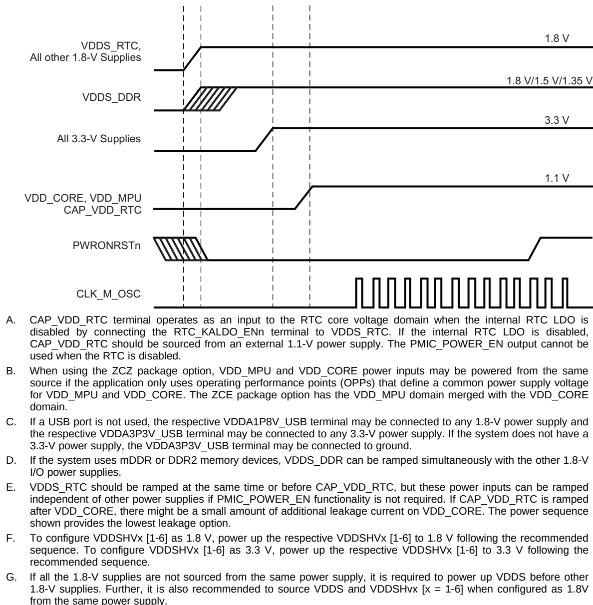
Figure 6-6. Power-Supply Sequencing With RTC Feature Disabled
