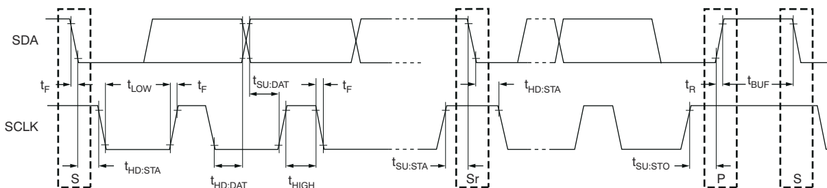
Figure 7-1. Timing Specification
