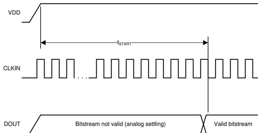
Figure 5-2. Device Start-Up Timing
