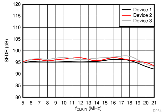
Figure 5-31. Spurious-Free Dynamic Range vs Input Clock Frequency
