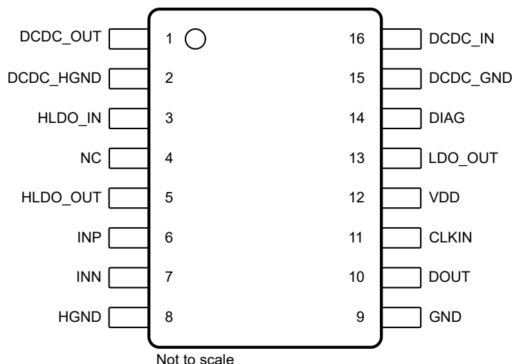
Figure 4-1. DWE Package, 16-Pin SOIC (Top View)
