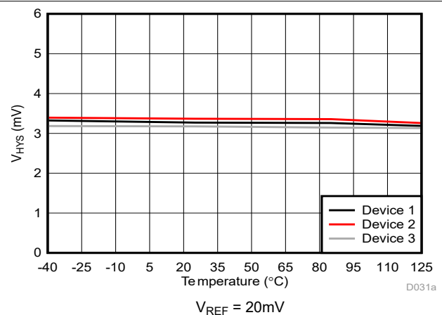
Figure 5-29. Cmp1 Trip Threshold Hysteresis vs Temperature
