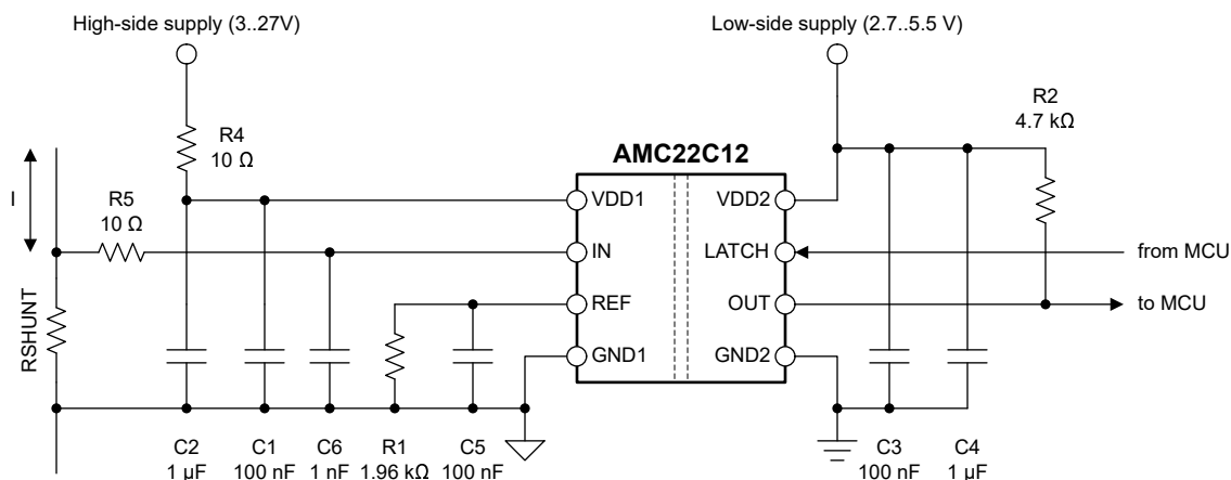
Figure 7-6. Decoupling of the AMC22C12
