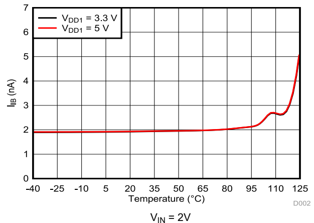
Figure 5-41. Input Bias Current vs Temperature
