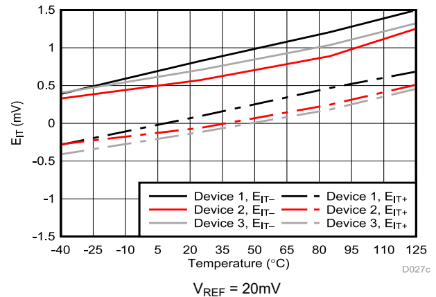
Figure 5-27. Cmp1 Trip Threshold Error vs Temperature
