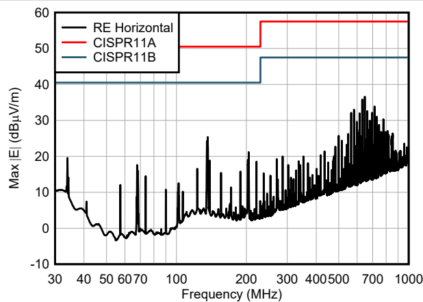
Figure 9-6. AMC130M02 Horizontal Radiated Emission CISPR11 Measurement
