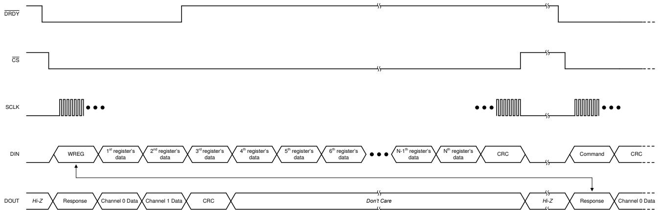
Figure 8-27. Writing Registers
