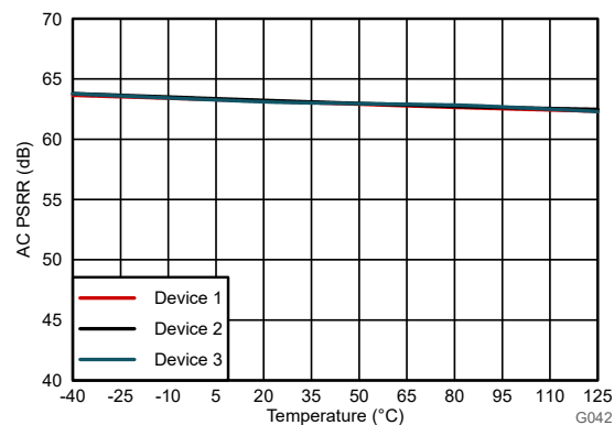
Figure 6-25. AC Power-Supply Rejection Ratio vs Temperature
