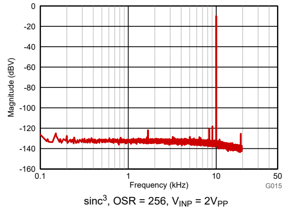
Figure 6-43. Frequency Spectrum With 10kHz Input Signal
