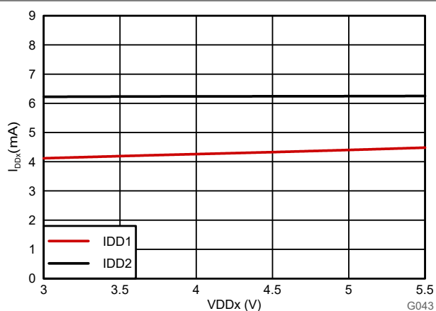
Figure 6-13. Supply Current vs Supply Voltage
