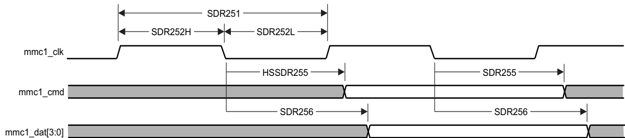
Figure 7-68. MMC/SD/SDIO in - High Speed SDR25 - Transmitter Mode
