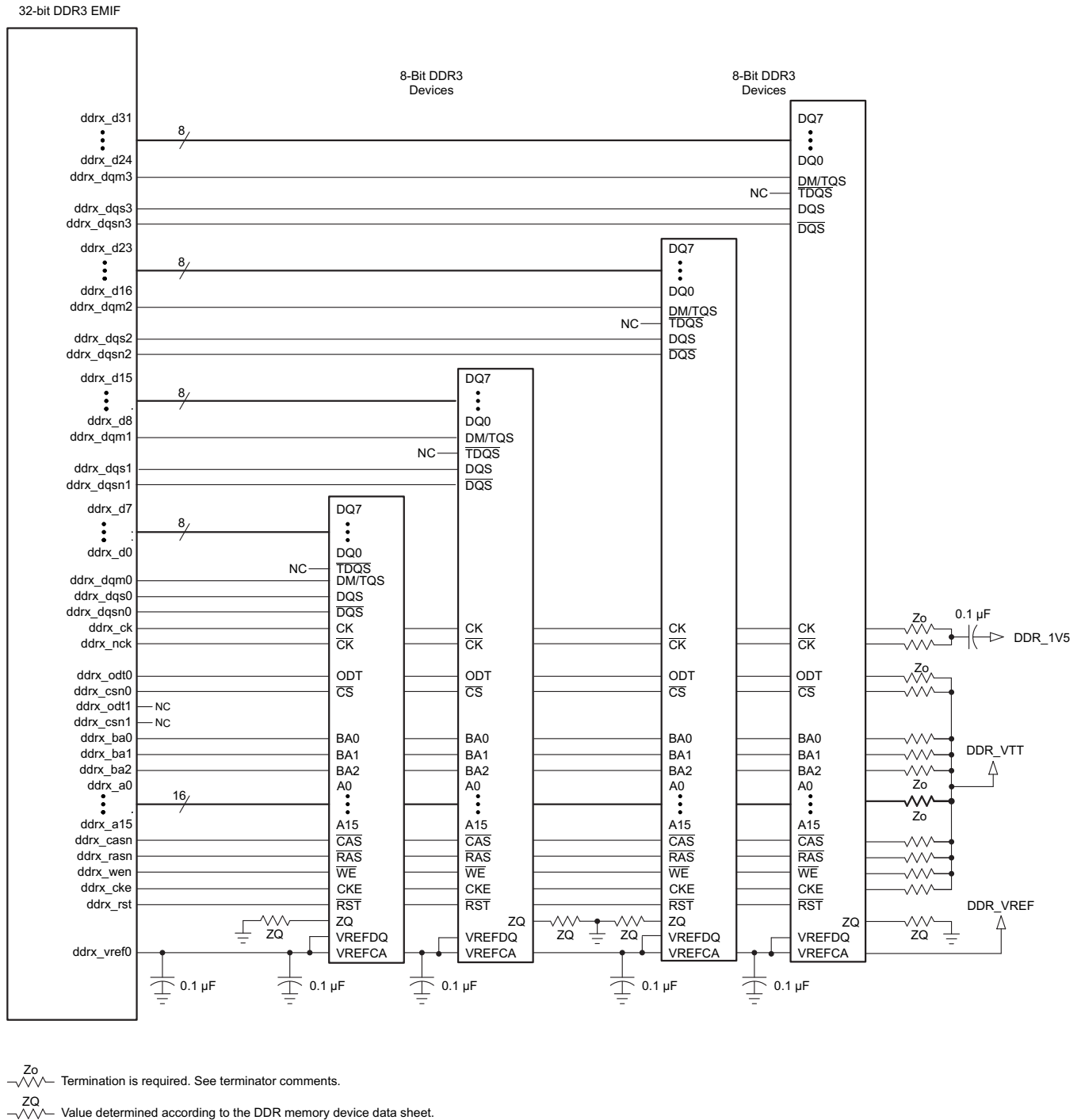
Figure 8-3. 32-Bit, One-Bank DDR3 Interface Schematic Using Four 8-Bit DDR3 Devices
