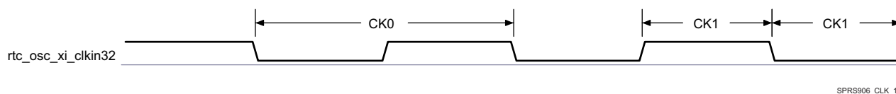
Figure 6-13. rtc_osc_xi_clkin32 Input Clock
