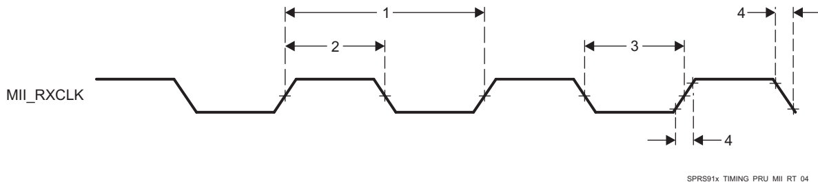
Figure 7-108. PRU-ICSS MII[x]_RXCLK Timing
