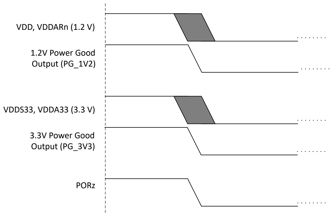
Figure 6-2. Power-Down Sequencing
