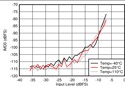
Figure 4-120. RX IMD3 vs Input Level and Temperature at 2.6 GHz
