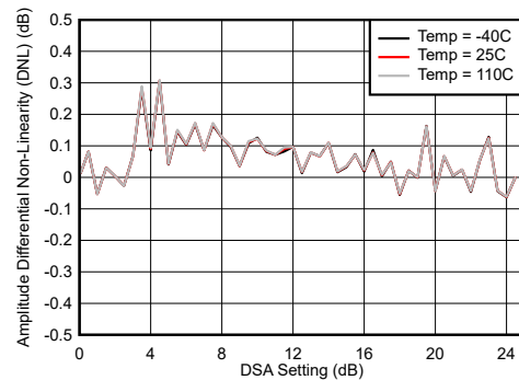
Differential Amplitude Error = P_{\text{IN}}(\text{DSA Setting} - 1) - P_{\text{IN}}(\text{DSA Setting}) + 1 Figure 4-2. RX Uncalibrated Differential Amplitude Error vs DSA Setting at 30 MHz
