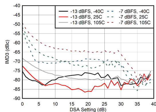
Figure 4-290. IMD3 vs DSA Setting at 400 MHz
