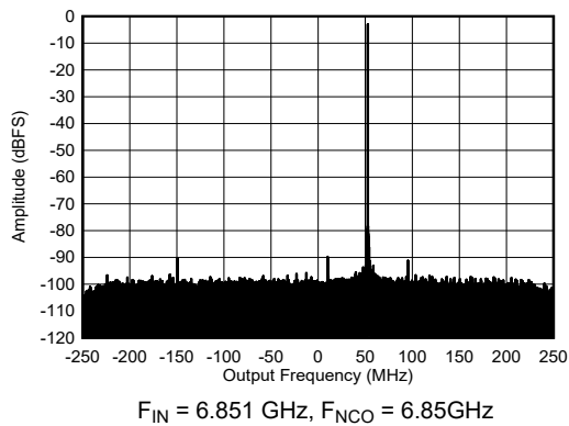
Figure 4-212. RX Output FFT at 6.851 GHz and -6 dBFS
