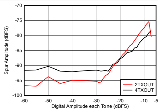
Inband = 3.75 GHz \pm 600 MHz, f_{\text{DAC}} = 9 GSPS, external clock mode, non-interleave mode.
