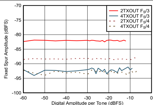
Inband = 2600 MHz \pm 600 MHz, f_{\text{DAC}} = 12 GSPS, external clock mode, non-interleave mode
