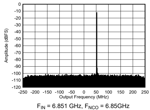
Figure 4-213. RX Output FFT at 6.851 GHz and -12 dBFS
