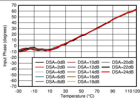
Figure 4-138. RX Input Phase vs Temperature at 3.6 GHz
