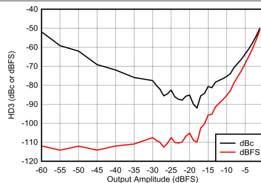
Figure 4-292. HD3 vs Amplitude at 400 MHz
