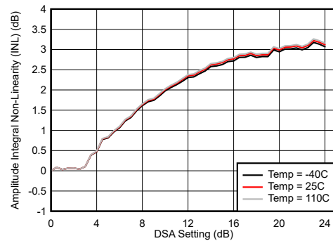
Integrated Amplitude Error = P_{\text{IN}}(\text{DSA Setting}) - P_{\text{IN}}(\text{DSA Setting} = 0) + (\text{DSA Setting}) Figure 4-4. RX Uncalibrated Integrated Amplitude Error vs DSA Setting at 30 MHz
