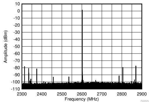
Figure 4-419. TX Single Tone (-6 dBFS) Output Spectrum at 2.6 GHz ( \pm 300 MHz)
