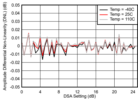
Differential Amplitude Error = P_{\text{IN}}(\text{DSA Setting} - 1) - P_{\text{IN}}(\text{DSA Setting}) + 1 Figure 4-3. RX Calibrated Differential Amplitude Error vs DSA Setting at 30 MHz
