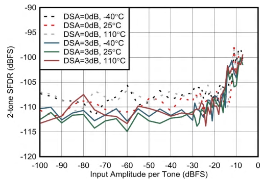
Figure 5-132. RX In-Band SFDR ( \pm 300\text{ MHz} ) vs Input Amplitude and Temperature at 2.6 GHz
