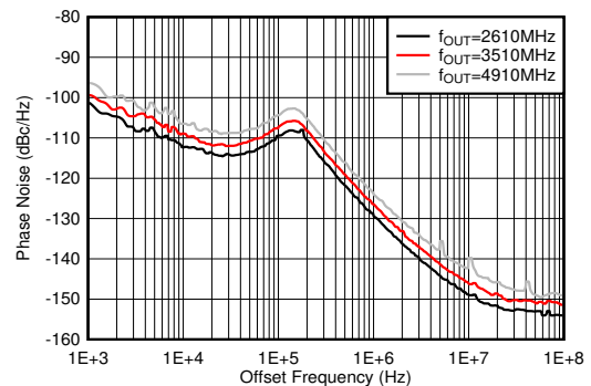
Figure 5-624. Phase Noise for 9-GHz VCO vs Offset Frequency and f_{OUT} at 25°C
