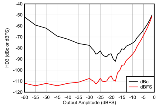
Figure 5-302. HD3 vs Amplitude at 400 MHz
