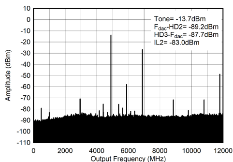
Figure 5-548. TX Single Tone (-6 dBFS) Output Spectrum at 4.9 GHz ( 0-f_{\text{DAC}} )
