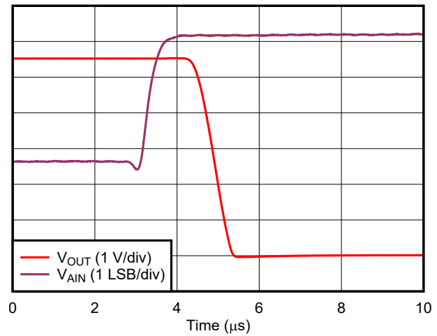
Figure 6-38. Comparator Response Time: High-to-Low Transition
