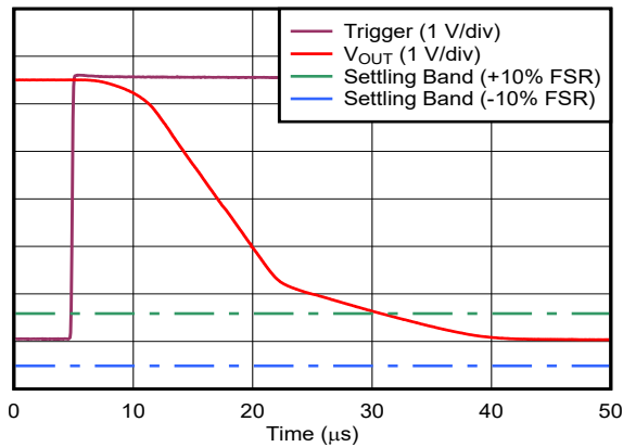
Figure 6-22. Voltage Output Setting Time - Falling Edge
