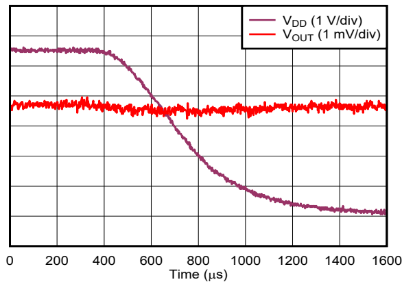
Figure 6-22. Voltage Output Setting Time - Falling Edge
