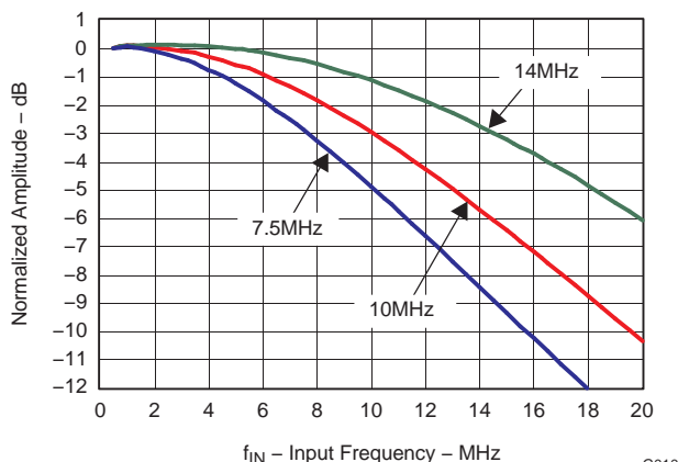
Figure 18. Antialiasing Filter Frequency Response
