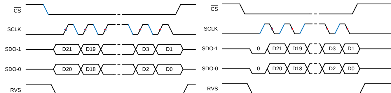
Figure 60. SPI-00-D Protocol
