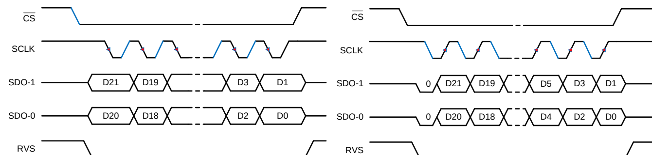
Figure 62. SPI-10-D Protocol
