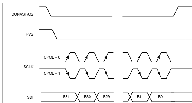
Figure 7-30. Standard SPI Timing Protocol (CPHA = 0, 32 SCLK Cycles)
