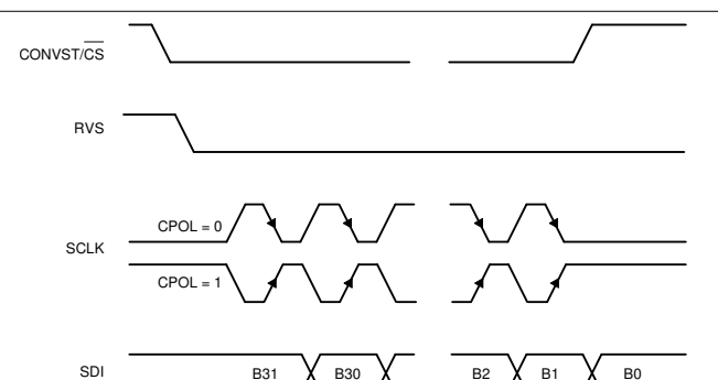
Figure 7-31. Standard SPI Timing Protocol (CPHA = 1, 32 SCLK Cycles)
