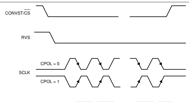
Figure 7-29. Standard SPI Timing Protocol (CPHA = 1, Single SDO-x)
