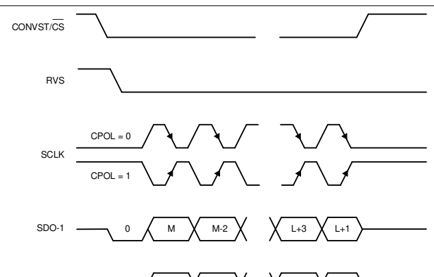
Figure 7-31. Standard SPI Timing Protocol (CPHA = 1, Dual SDO-x)
