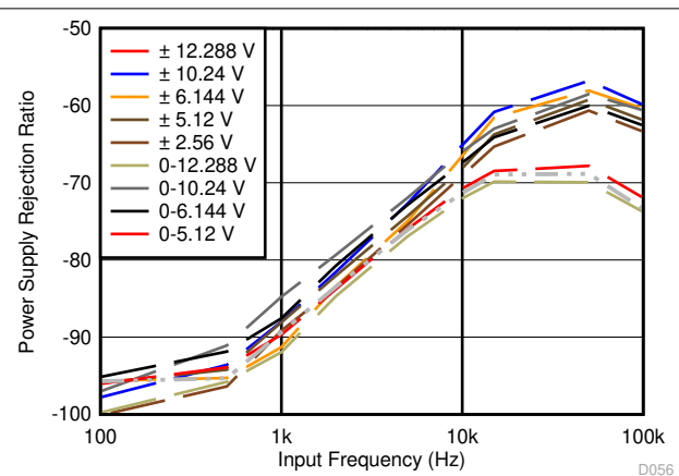
Figure 9-2. PSRR With a Decoupling Capacitor
