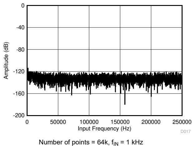
Figure 6-34. Typical FFT Plot (All Ranges) for the ADS8675
