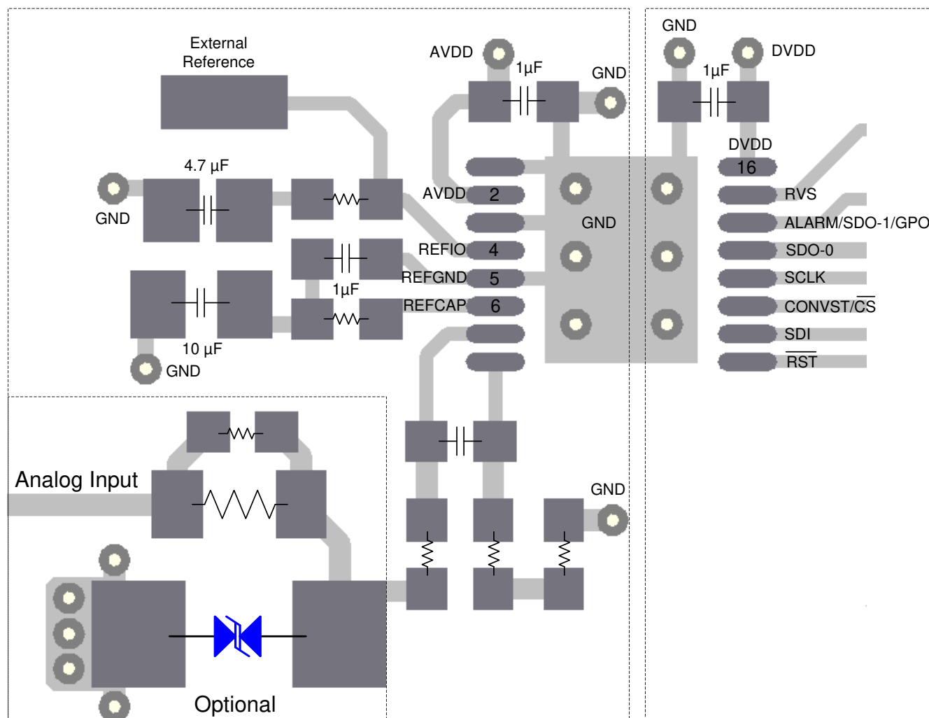
Figure 10-1. Board Layout for the ADS867x
