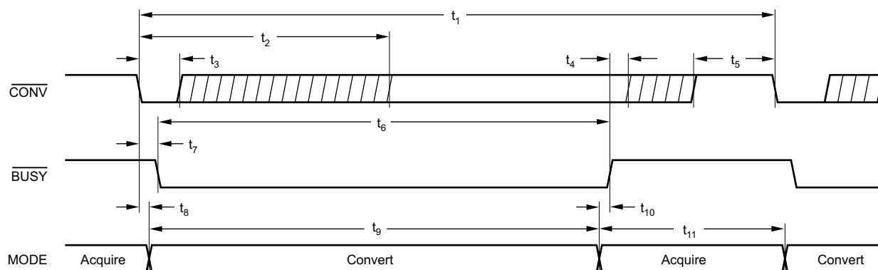
Figure 36. Basic Conversion Timing
