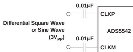
Figure 45. AC-Coupled, Differential Clock Input
