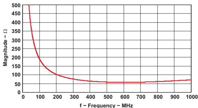
Figure 36. Input Impedance, Z_1
