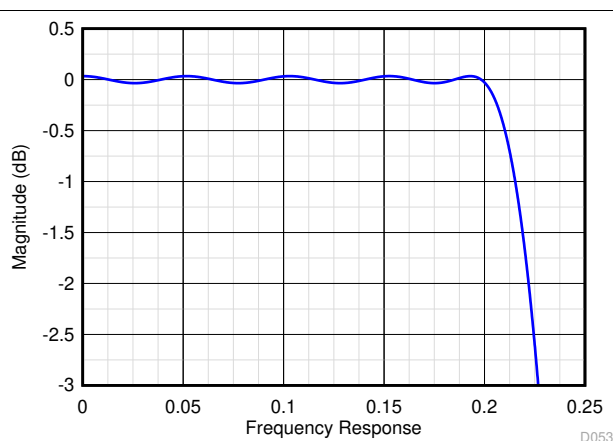
Figure 7-5. Zoomed View of Frequency Response
