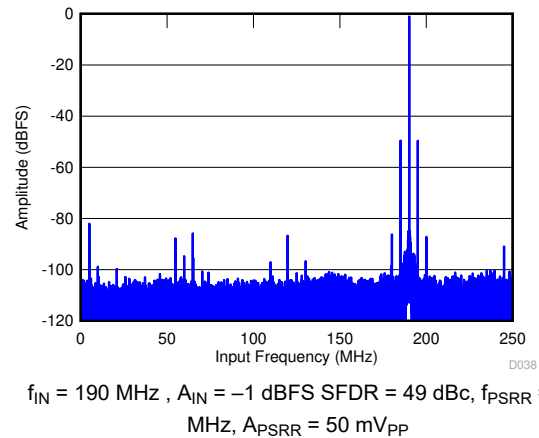
Figure 6-40. Power-Supply Rejection Ratio FFT for Test Signal on AVDD Supply
