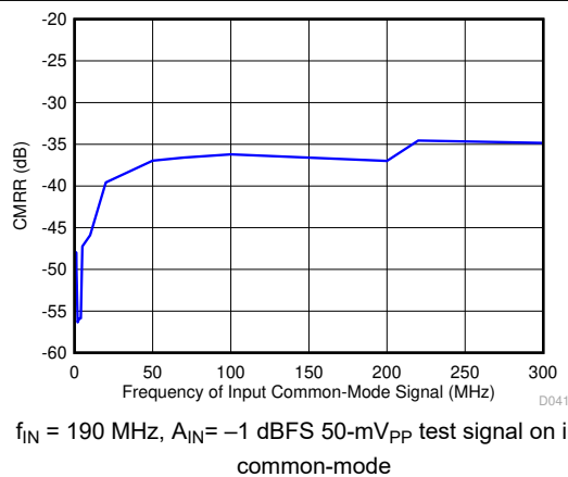
Figure 6-43. Common-Mode Rejection Ratio
