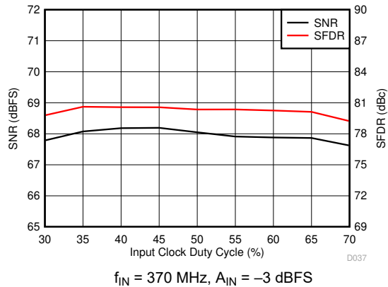
Figure 6-39. Performance vs Clock Duty Cycle
