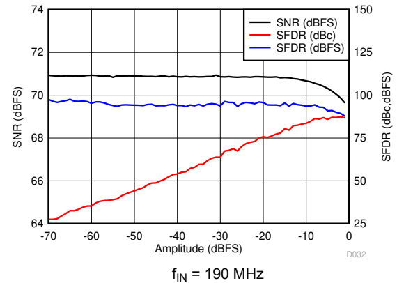
Figure 6-34. Performance vs Amplitude
