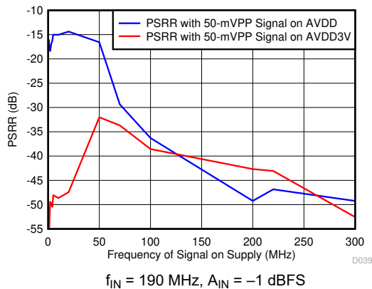
Figure 6-41. Power-Supply Rejection Ratio vs Supplies
