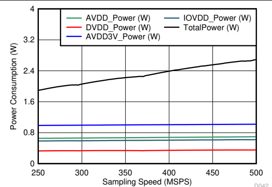
Figure 6-44. Power vs Chip Clock
