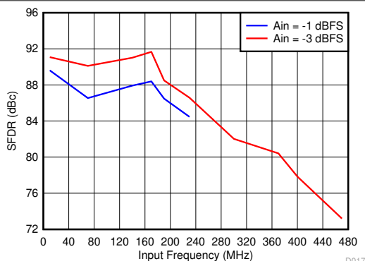
Figure 6-19. Spurious-Free Dynamic Range vs Input Frequency
