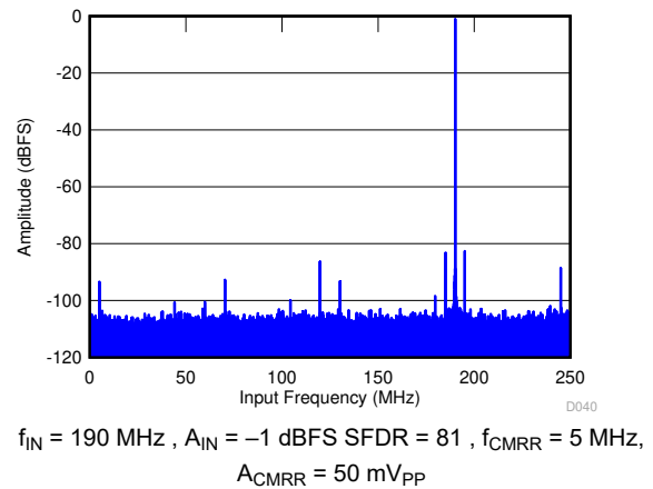
Figure 6-42. Common-Mode Rejection Ratio FFT
