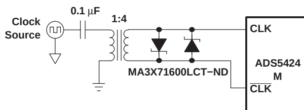
Figure 22. Differential Clock
