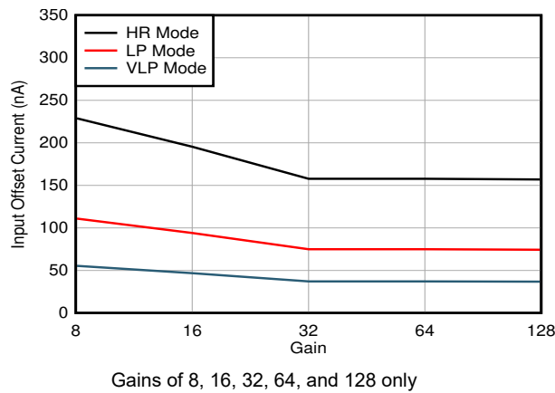
Figure 6-4. Input Offset Current vs Gain
