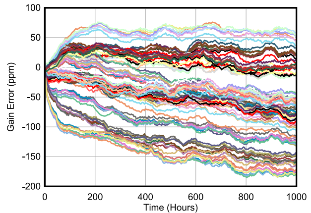
Figure 6-11. Long-Term Gain Drift (WQFN Package)
