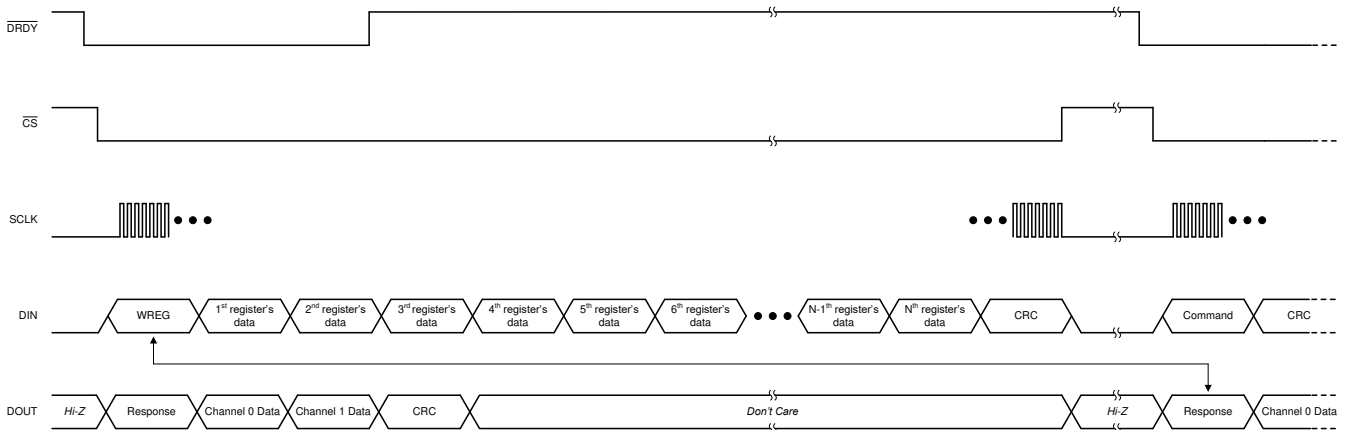
Figure 8-23. Writing Registers
