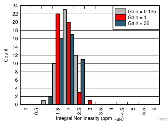
Figure 7-12. Nonlinearity Distribution
