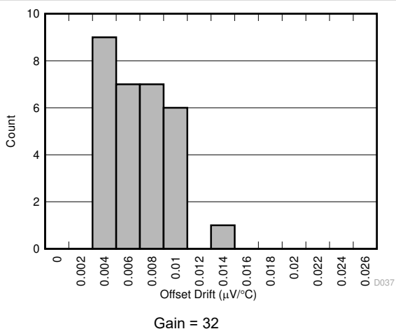
Figure 7-15. Offset Error Drift Distribution
