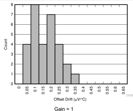
Figure 7-14. Offset Error Drift Distribution
