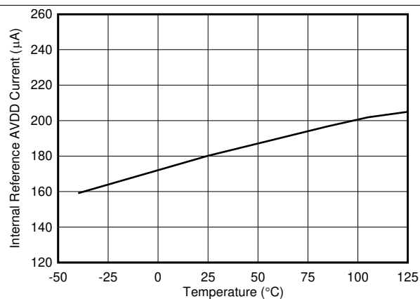
Figure 38. Internal Reference AVDD Current vs Temperature
