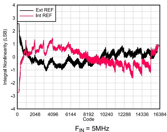
Figure 5-23. INL vs Code
