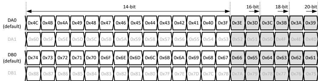
Figure 7-38. 1-wire output bit mapping
