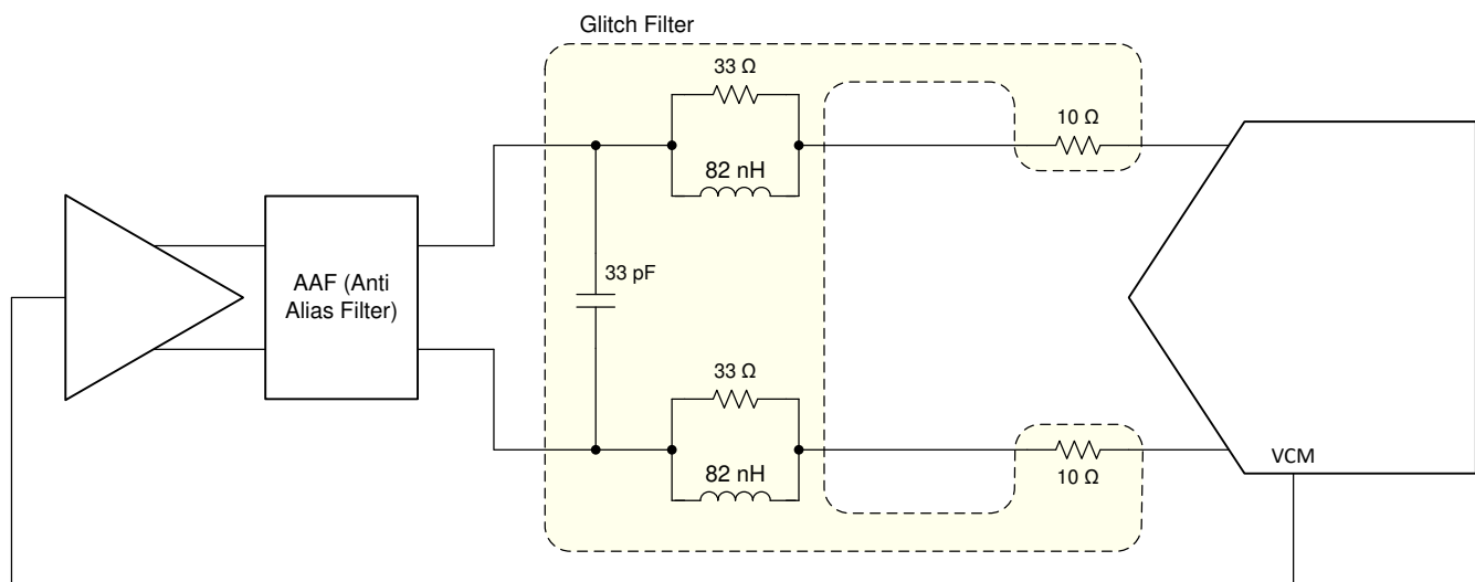
Figure 7-7. DC-Coupling: DC bias provided by FDA (glitch filter example for DC - 60MHz)
