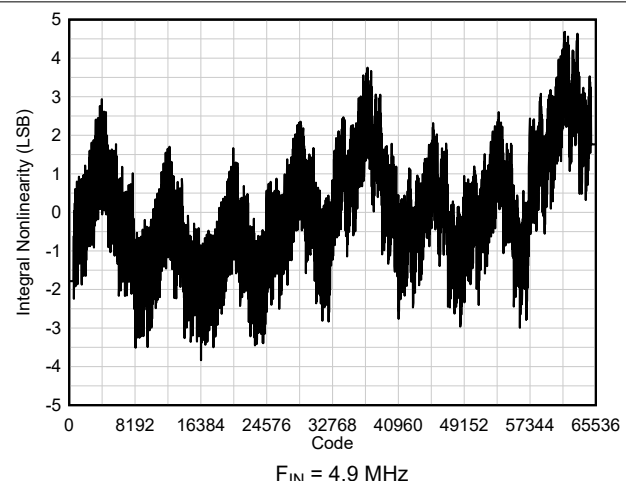
Figure 6-12. INL vs Code
