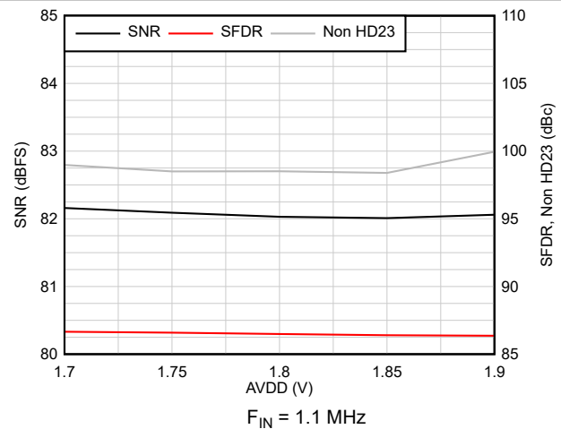
Figure 6-10. AC Performance vs AVDD
