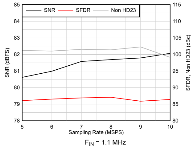
Figure 6-8. AC Performance vs Sampling Rate
