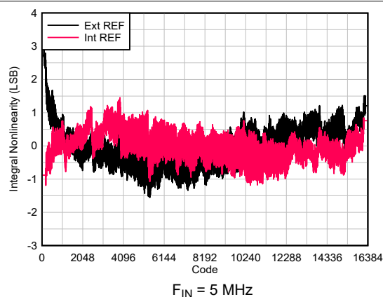
Figure 6-20. INL vs Code
