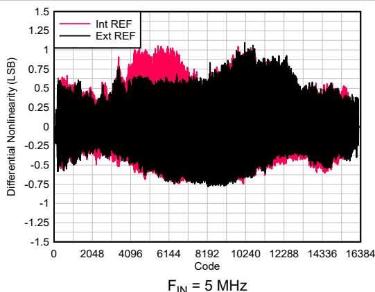
Figure 6-21. DNL vs Code
