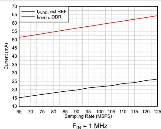
Figure 6-24. Current vs Sampling Rate
