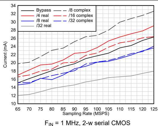
Figure 6-25. I_{IOVDD} Current vs Decimation
