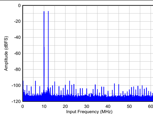
Figure 6-8. Two Tone FFT at F_{IN} = 10/12\text{ MHz}
