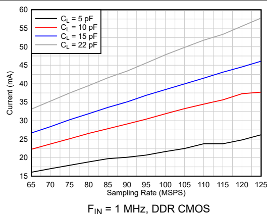
Figure 6-26. I_{IOVDD} Current vs Load Capacitance
