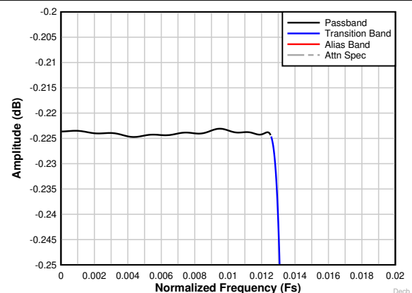
Figure 8-29. Decimation by 32 complex passband ripple response
