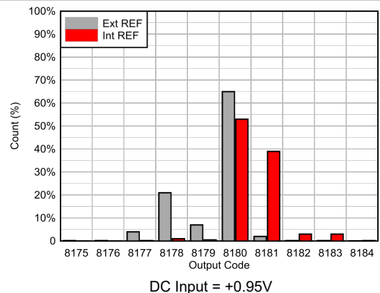
Figure 6-22. DC Offset Histogram
