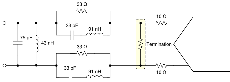
Figure 8-5. Sampling glitch filter example for input frequencies from 60 to 120 MHz
