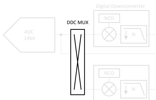
Figure 8-22. DDC MUX
