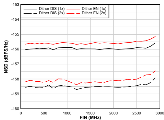
A_{IN} = -20\text{ dBFS} Figure 5-26. NSD Performance vs F_{IN}
