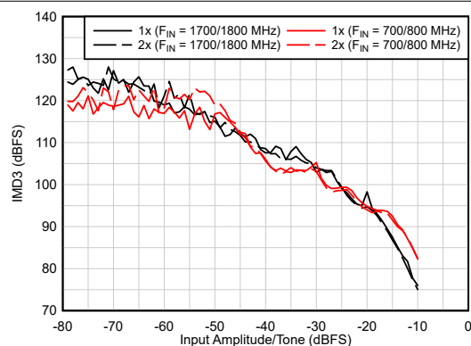
Dither = EN Figure 5-30. IMD3 Performance vs A_{IN}
