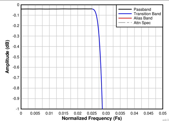
Figure 6-29. Decimation by 16 Passband Ripple Response
