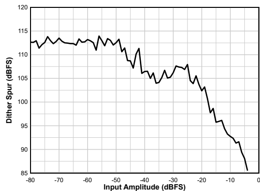
F_{IN} = 900\text{ MHz} , Figure 5-25. Dither Spur vs A_{IN}
