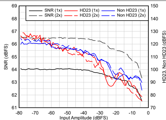
F_{IN} = 900\text{ MHz} , Dither = EN Figure 5-28. AC Performance vs A_{IN}
