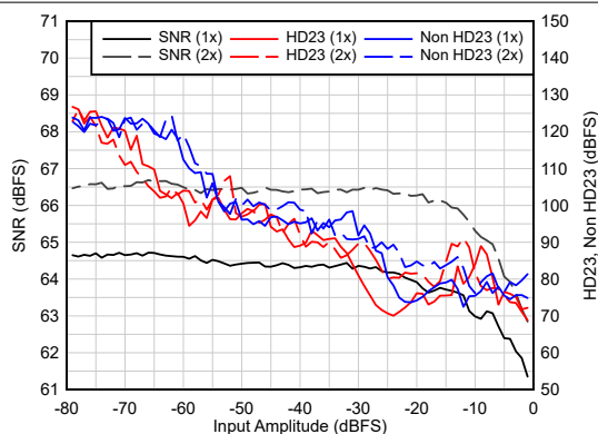
F_{IN} = 900\text{ MHz} , Dither = DIS Figure 5-27. AC Performance vs A_{IN}
