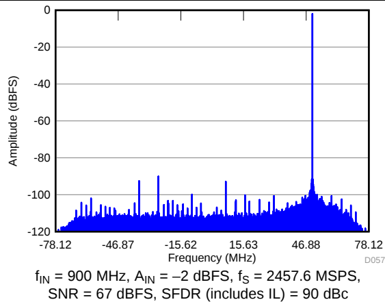
Figure 59. FFT in 16x Decimation (Complex Output)
