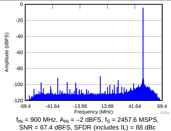
Figure 60. FFT in 18x Decimation (Complex Output)
