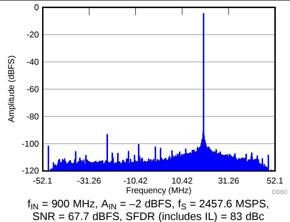
Figure 62. FFT in 24x Decimation (Complex Output)
