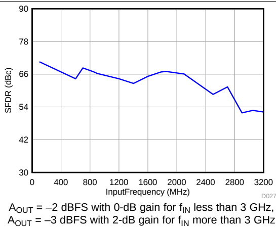
Figure 29. Spurious-Free Dynamic Range vs Input Frequency ( f_s = 2211.84 \text{ MSPS} )
