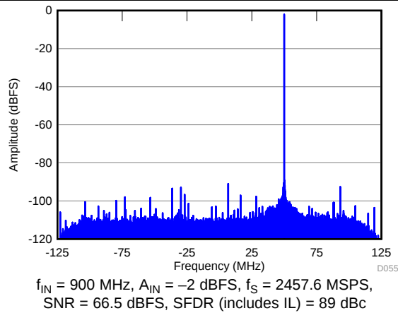
Figure 57. FFT in 10x Decimation (Complex Output)
