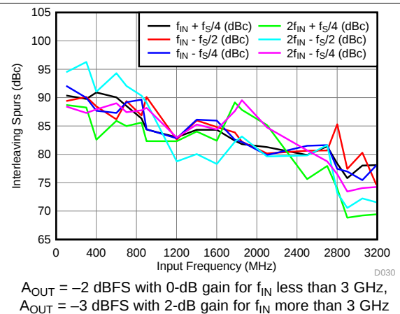
Figure 32. IL Spur vs Input Frequency ( f_s = 2211.84 \text{ MSPS} )
