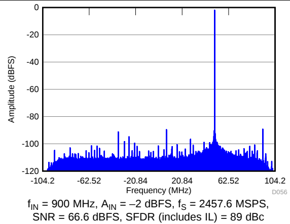
Figure 58. FFT in 12x Decimation (Complex Output)
