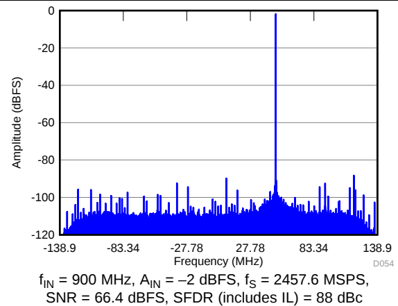
Figure 56. FFT in 9x Decimation (Complex Output)
