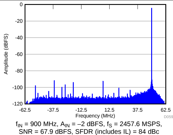
Figure 61. FFT in 20x Decimation (Complex Output)
